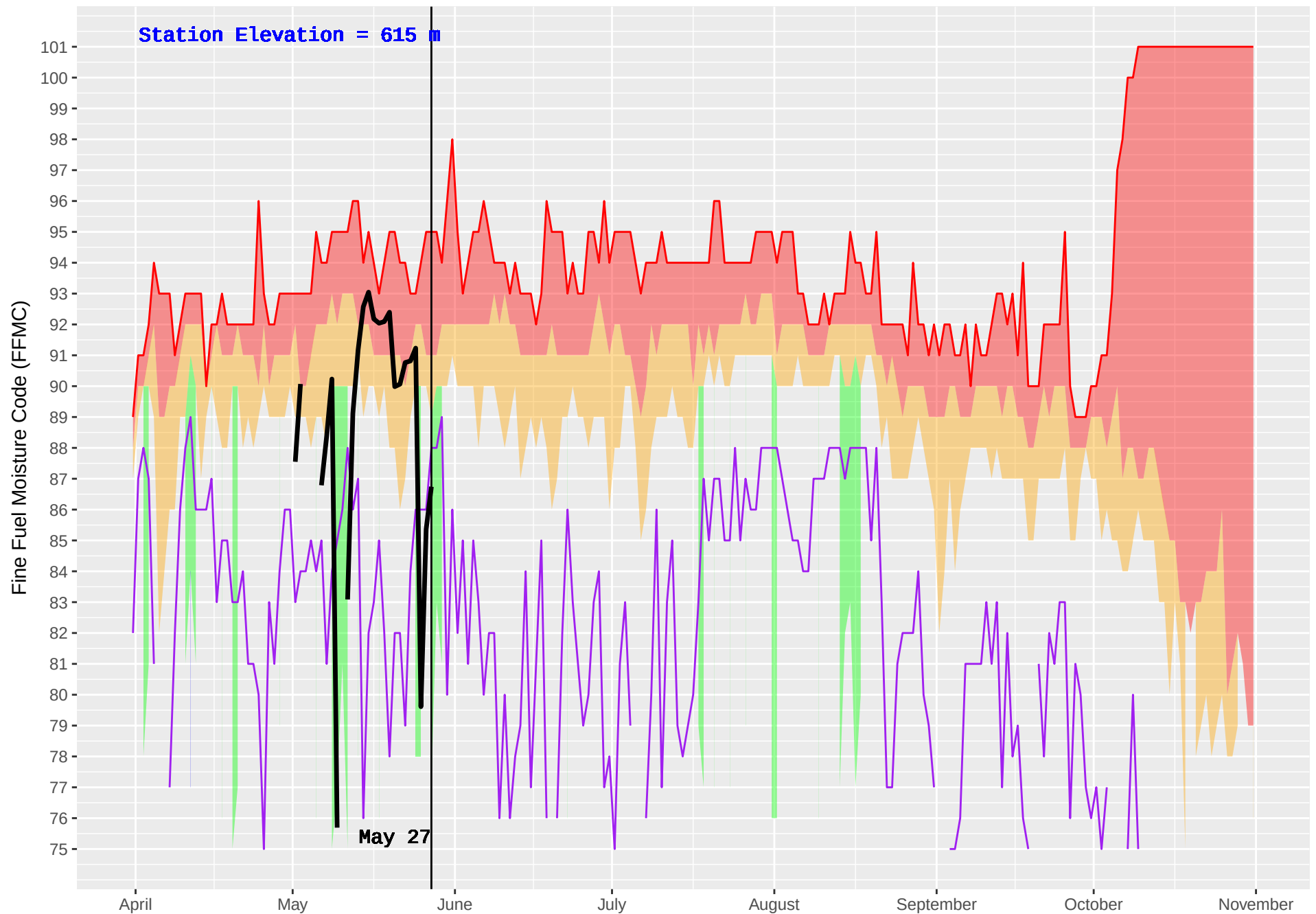
HIXON (187) : Historical (1976–2016) and Current (2018) Noon Fine Fuel Moisture Code (FFMC)
